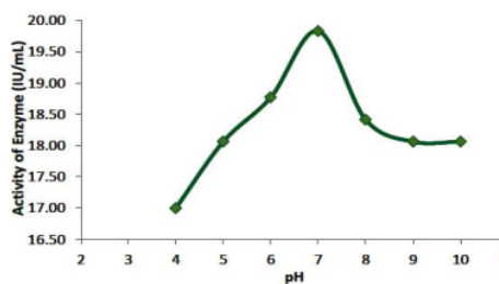
7 Fig. 4. Effect of pH on the enzyme activity of L - Asparaginase at 37 °C.
